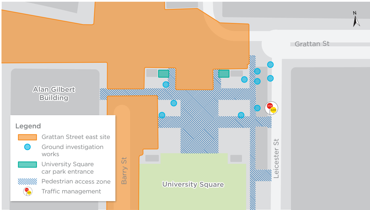
Ground investigation locations, Parkville. Indicative only
