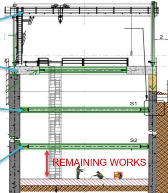
Artists impression of retrieval shaft
